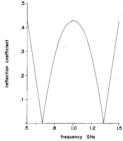
Fig. 3. The minimax response of the two-section transformer.
