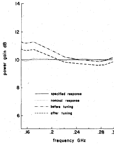
Fig. 7. The results of tuning an outcome corresponding to vertex number 123 of the broad-band amplifier using the modeling technique.
